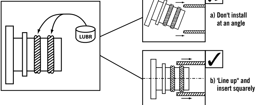
Figure 3. Lubricate gaskets with WRAS approved lubricant
